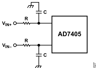
Figure 27. RC Low-Pass Filter Input Network
