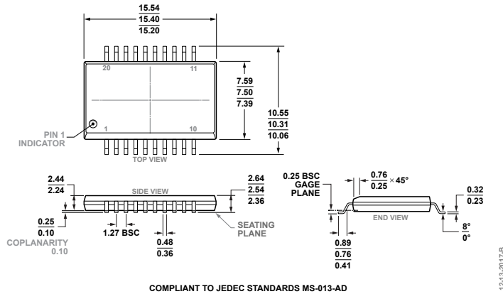
Figure 59. 20-Lead Standard Small Outline Package, with Increased Creepage [SOIC_IC] Wide Body (RI-20-1) Dimensions shown in millimeters
