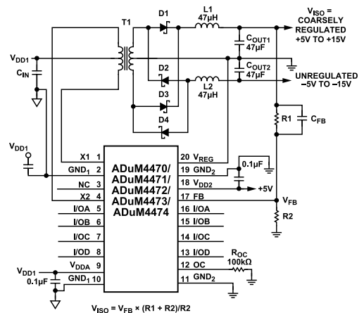
Figure 50. Positive and Unregulated Negative Supply
