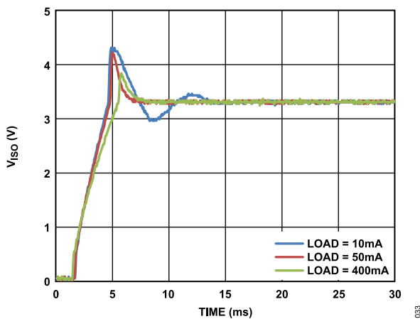
Figure 33. Typical V_{ISO} Startup 5 V Input to 3.3 V Output with 10 mA, 50 mA, and 400 mA Output Load
