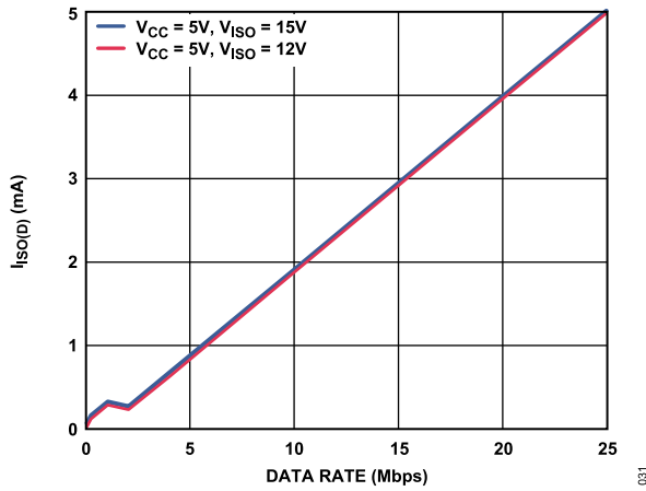
Figure 31. Typical Double-Supply I_{ISO(D)} Dynamic Supply Current per Input Channel
