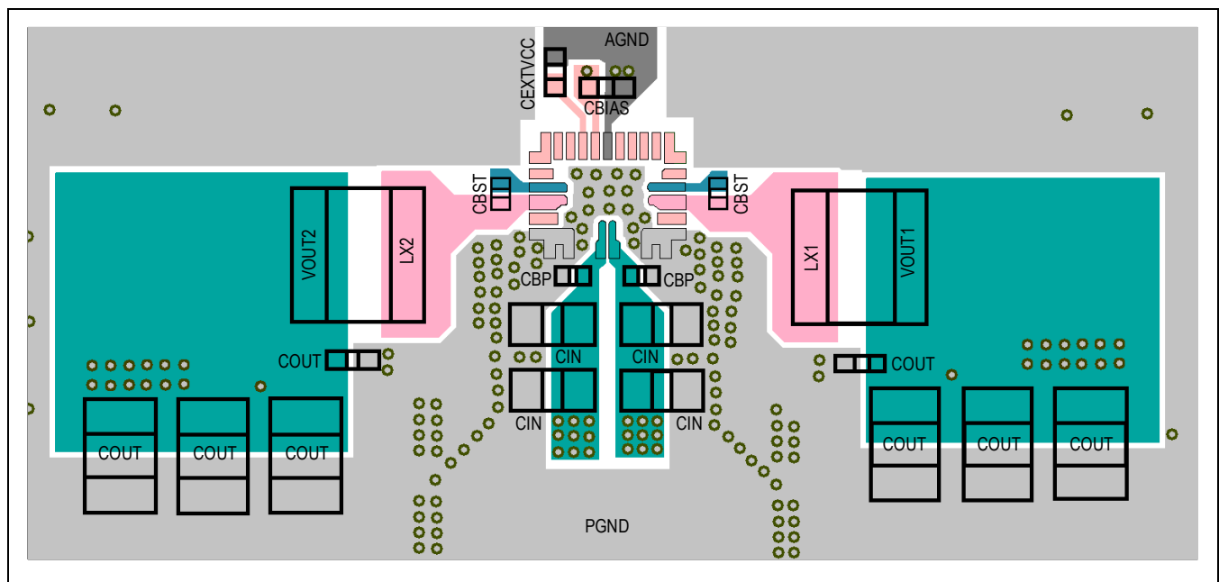
Figure 2. Layout Example
