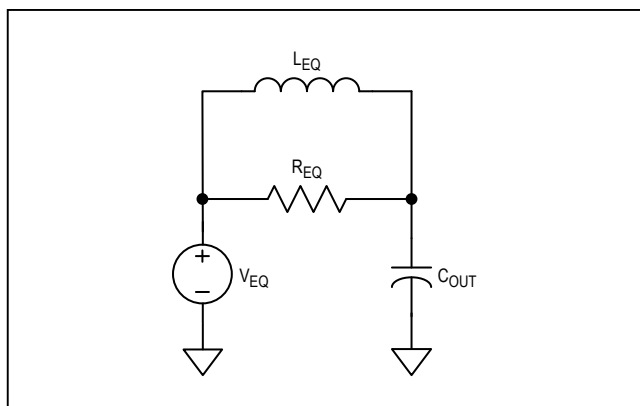
Figure 7. Averaged Small-Signal Equivalent Circuit of Regulator
