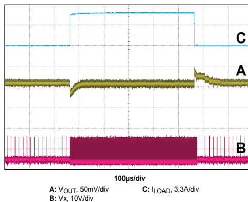
Unload-Transient Response DCM – Zoom In
