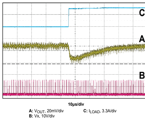
Load-Transient Response CCM – Zoom In
