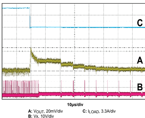
Negative Overcurrent Protection
