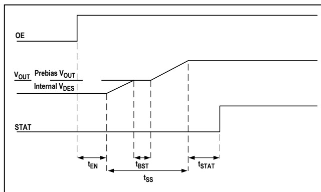
Figure 1. Startup Timing
