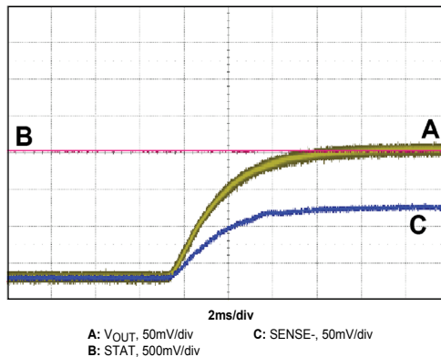
Startup with V_{CC} , External V_{REF}
