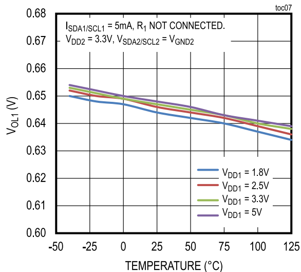
SIDE 1 OUTPUT LOW VOLTAGE vs. TEMPERATURE
