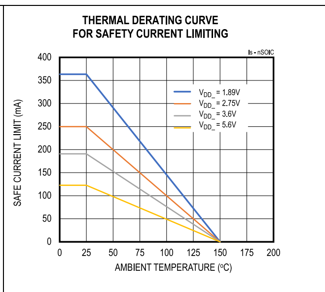
Figure 4. Thermal Derating Curve for Safety Current Limiting for 8-Lead Narrow SOIC (21-0041) Package
