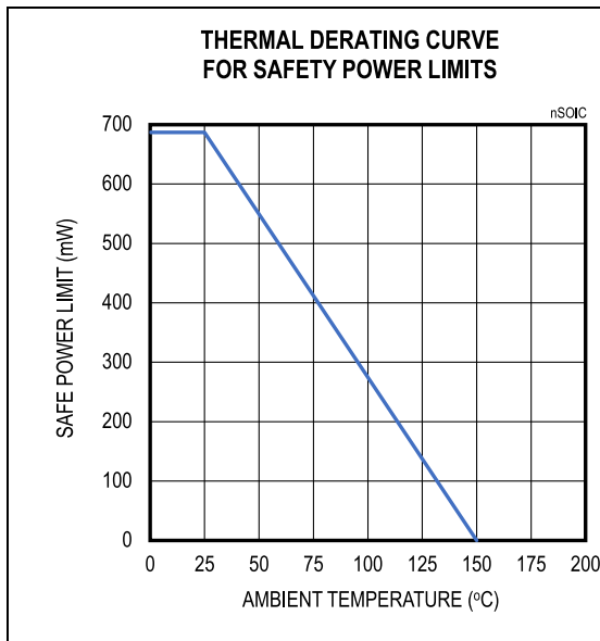
Figure 3. Thermal Derating Curve for 8-Lead Narrow SOIC (21-0041) Package
