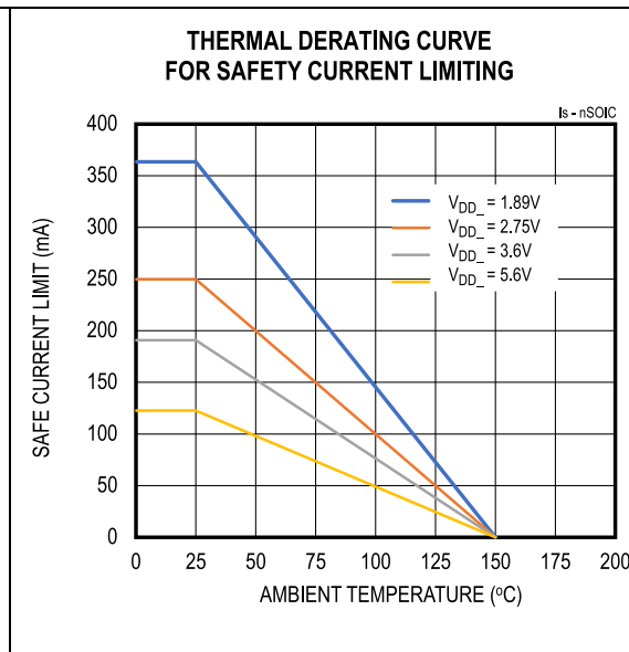
Figure 4. Thermal Derating Curve for Safety Current Limiting for 8-Lead Narrow SOIC (21-0041) Package
