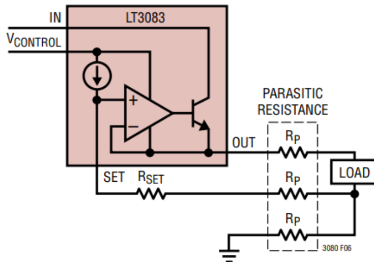
Figure 3 - Connections for Best Load Regulation
