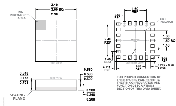
Figure 28. 24-Terminal Land Grid Array [LGA] (CC-24-14)
