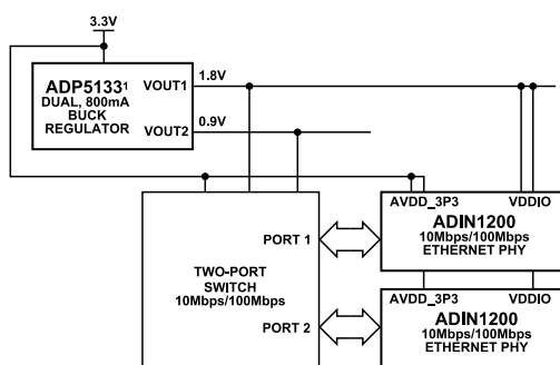
Figure 40. Recommended Power Solution for 3.3 V with RGMII Operating at VDDIO = 1.8 V
