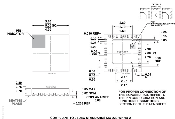
Figure 45. 32-Lead Lead Frame Chip Scale Package [LFCSP] 5 mm × 5 mm Body and 0.75 mm Package Height (CP-32-31) Dimensions shown in millimeters
