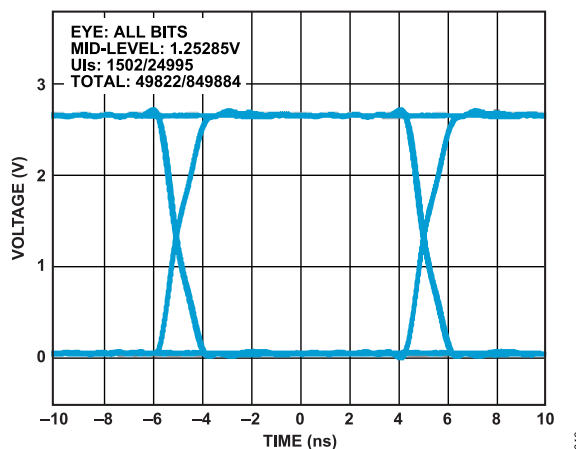
Figure 19. ADuM321N Eye Diagram
