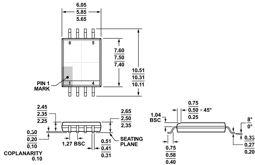
Figure 22. 8-Lead Standard Small Outline Package, with Increased Creepage [SOIC_IC] Wide-Body (Rl-8-1)
