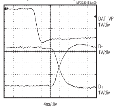
DRIVER PROPAGATION DELAY HIGH-TO-LOW (FULL-SPEED MODE)
