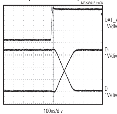
DRIVER PROPAGATION DELAY LOW-TO-HIGH (LOW-SPEED MODE)
