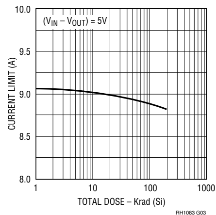
Current Limit
