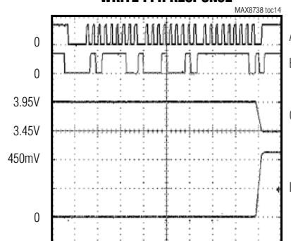
WRITE FFH RESPONSE
