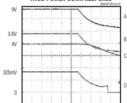
AVDD POWER-DOWN RESPONSE
