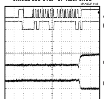
SINGLE LSB STEP-UP RESPONSE
