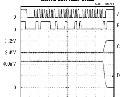
WRITE 00H RESPONSE
