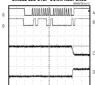
SINGLE LSB STEP-DOWN RESPONSE
