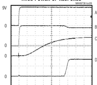
AVDD POWER-UP RESPONSE
