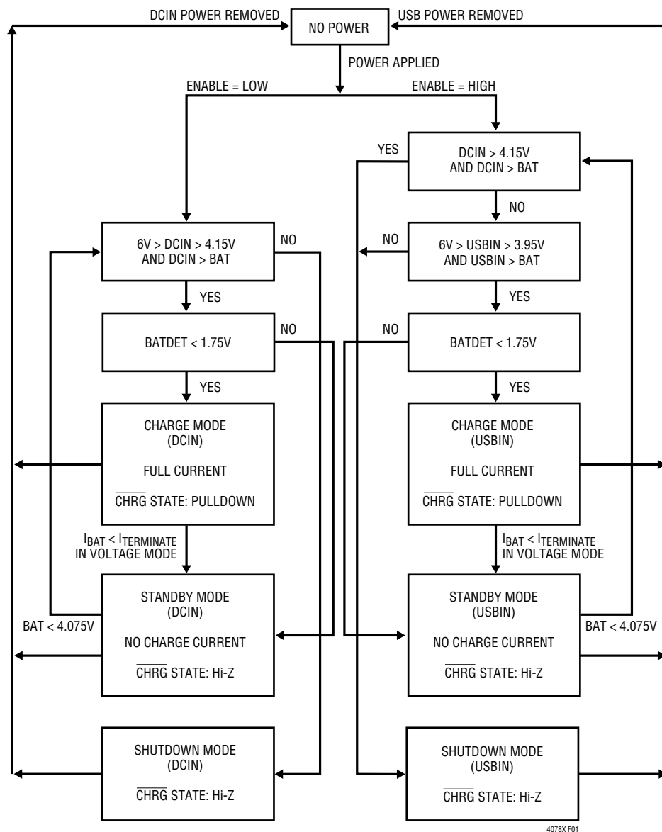
Figure 1. LTC4078X State Diagram of a Charge Cycle
