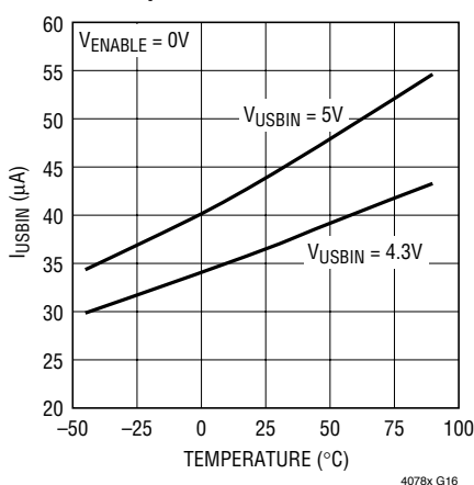
USBIN Shutdown Current vs Temperature
