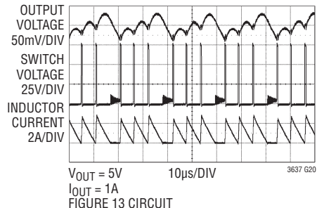
Operating Waveforms, V_{IN} = 76V
