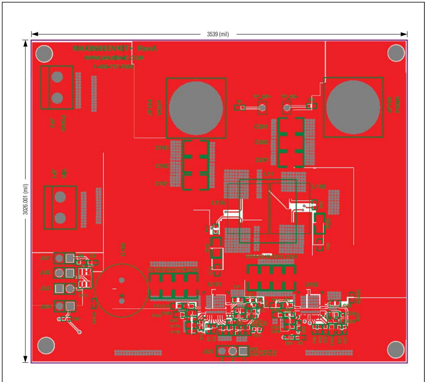
Figure 3. MAX8686 EV Kit PCB Layout—Component Side
